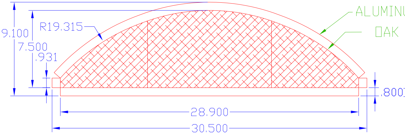
FRONT SIDE HAMMERFORM TEMPLATE
