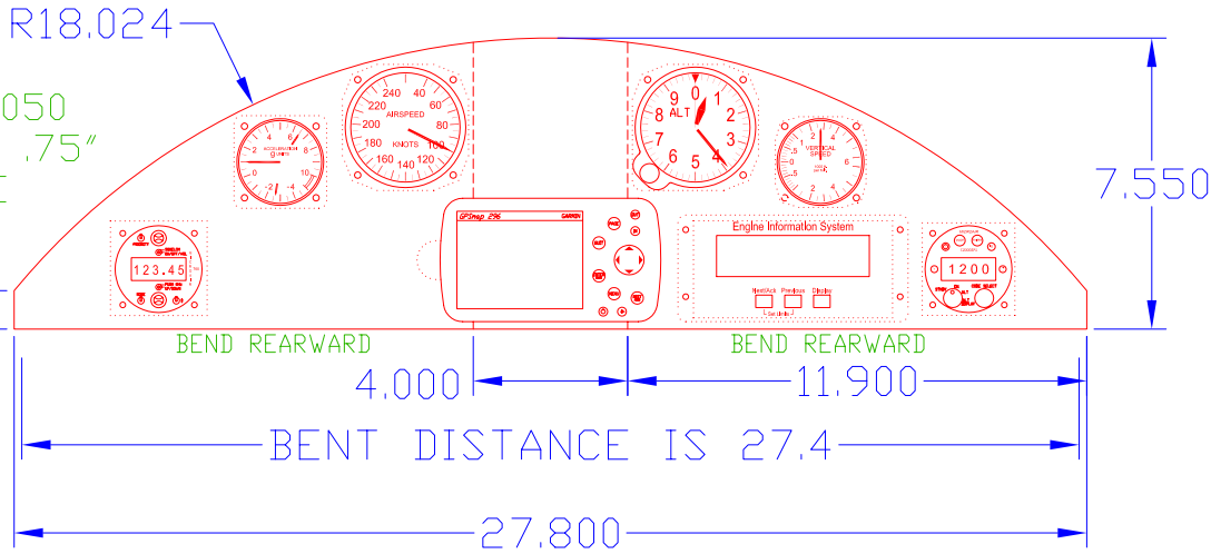
REAR SIDE OF REAR INSTRUMENT PANEL
