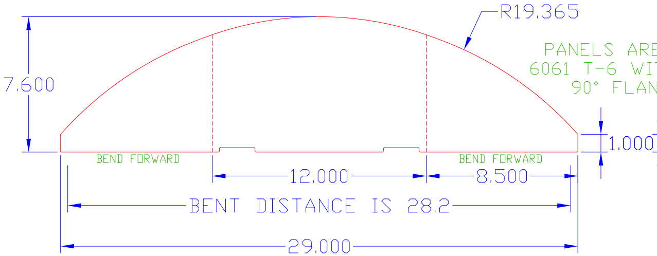
FRONT SIDE OF REAR INSTRUMENT PANEL
