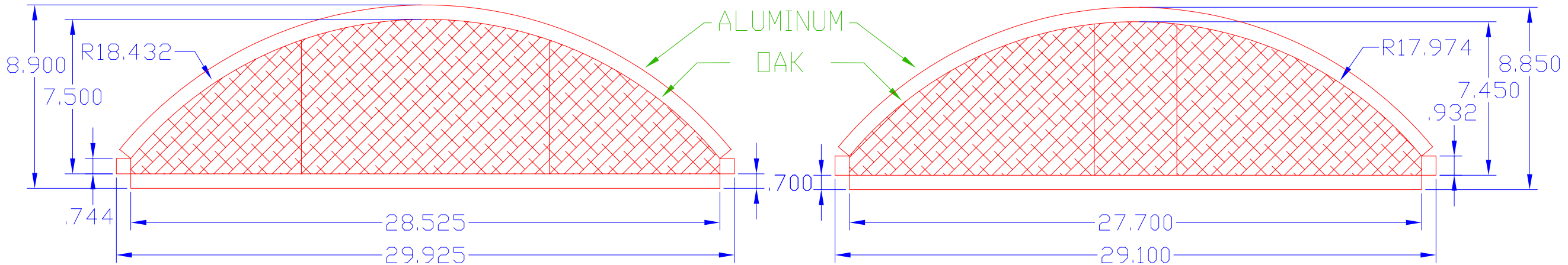
FRONT SIDE HAMMERFORM TEMPLATE
