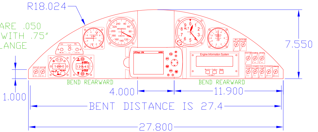
REAR SIDE OF REAR INSTRUMENT PANEL
